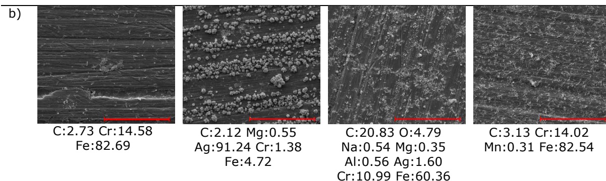
Figure 2. SEM micrographs (mag.3500 x) showing the aspect of 430 AISI stainless steel coupons a) before and b) after exposure to P. aeruginosa culture and EDX analysis. Scale bar: 40 \mu\text{m} . EDX values are in percentage.
