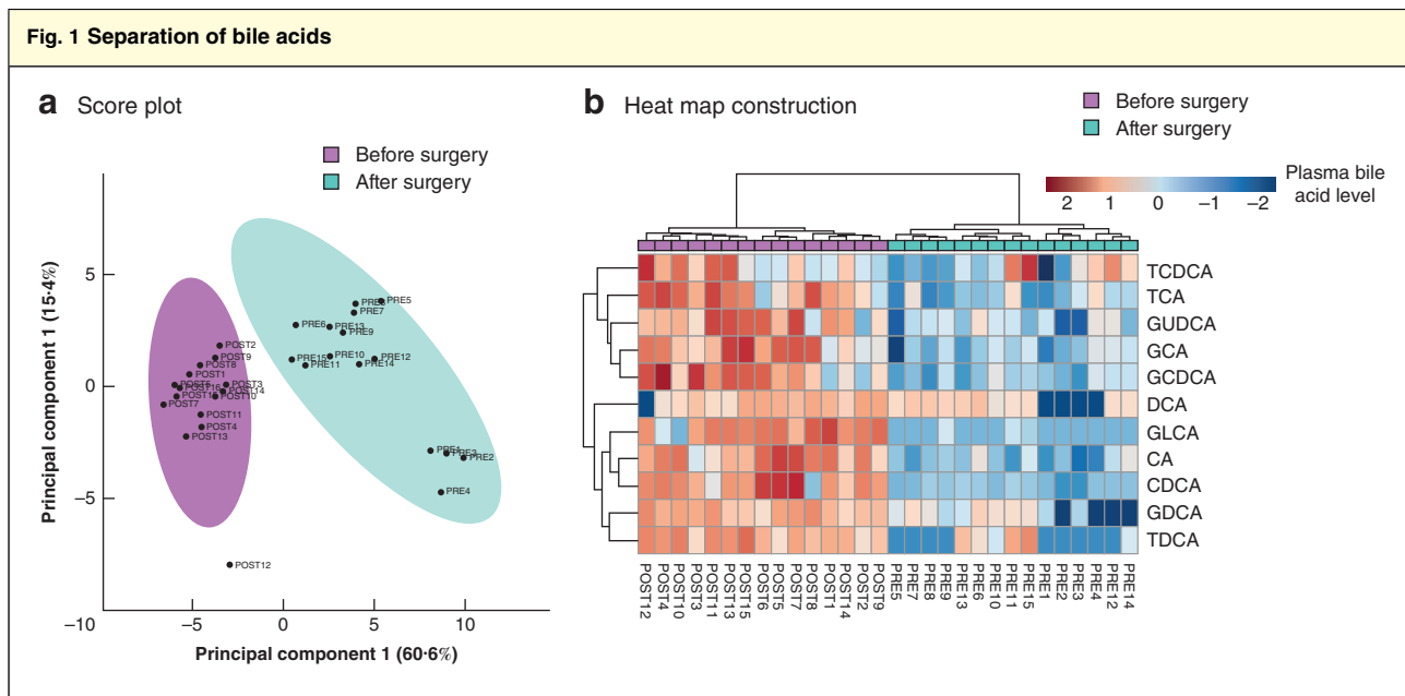
a Score plot of the two principal components from the principal component analysis. b Heat map with clustering analysis on autoscaled features. POST, after surgery; PRE, before surgery; TCDC A, taurochenodeoxycholic acid; TCA, taurocholic acid; GUDCA, glyoursodeoxycholic acid; GCA, glycocholic acid; GCDCA, glycochenodeoxycholic acid; DCA, deoxycholic acid; GLCA, glycolithocholic acid; CA, cholic acid; CDCA, chenodeoxycholic acid; GDCA, glycodeoxycholic acid; TDCA, taurodeoxycholic acid.
