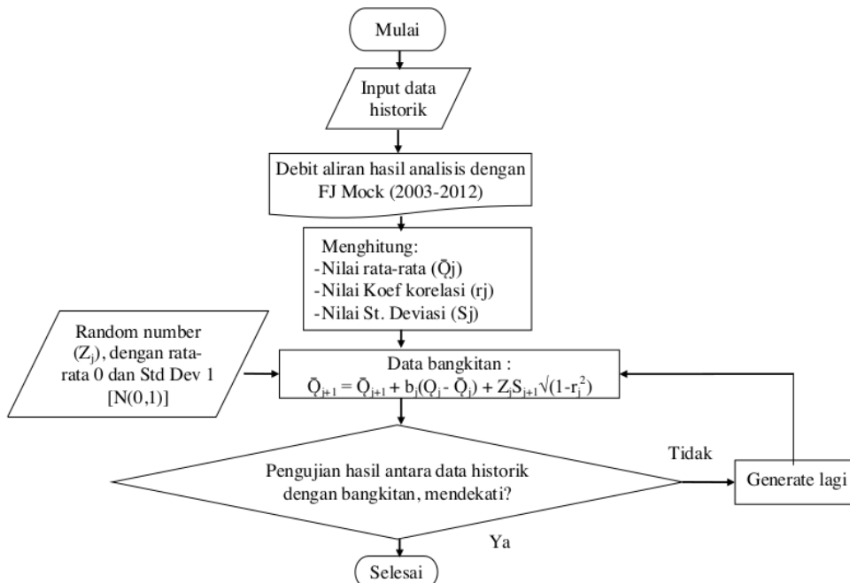
Gambar 2. Peramalan data Model Thomas Fierin
