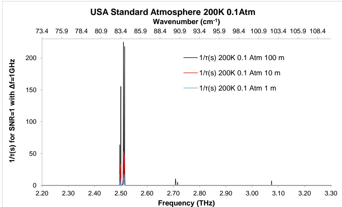
Fig. 6.13: Maximum sampling rate for chain 0 for a path of, respectively, 1\text{m} , 10\text{m} , 100\text{m} in a homogeneous medium. The chart has been generated using a standard atmosphere at 200\text{K} and 0.1\text{Atm} pressure (corresponding to high tropospheric conditions).
