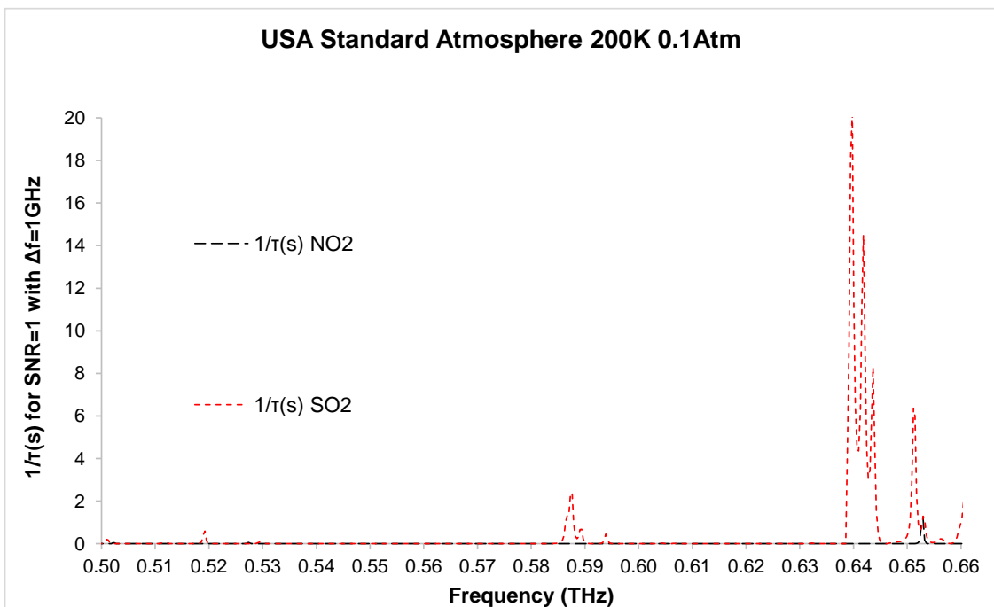
Fig. 6.17: Maximum sampling rate for the species observed by Chain 1 instrument for a 10 \text{ m} path in high tropospheric conditions. The species providing no detectable signal have been excluded from the chart.
