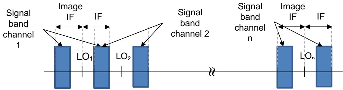
Fig. 5.2: non-fixed (tuneable) LO, using a narrow IF band. The system acquires a signal in DSB.
