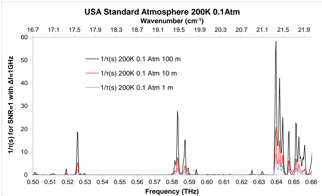
Fig. 6.16: Maximum sampling rate for chain 1 for having SNR = 1 and \Delta\nu = 1 \text{ GHz} for a path of, respectively, 1\text{m} , 10\text{m} , 100\text{m} in a homogeneous medium, as in Fig. 6.12. The chart has been generated using a standard atmosphere at 200\text{K} and 0.1 \text{ Atm} pressure (high tropospheric conditions).
