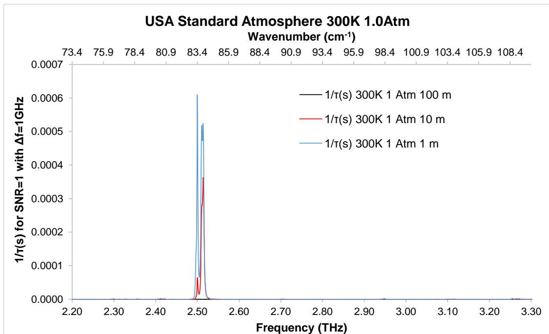
Fig. 6.12: Maximum sampling rate for chain 0 for having SNR = 1 and \Delta\nu = 1\text{GHz} for a path of, respectively, 1\text{m} , 10\text{m} , 100\text{m} in a homogeneous medium. Higher is the value, shorter is the corresponding integration time \Delta\tau_{int} . The sampling rate scales with the SNR square value and is inversely proportional to \Delta\nu . The chart has been generated using a standard atmosphere at 300\text{K} and 1.0\text{Atm} pressure (corresponding to sea level conditions).
