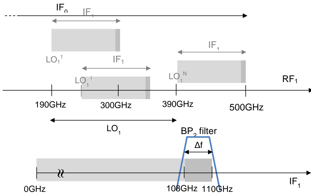
Fig. 5.5: Stage 1: A variable local oscillator LO 1 can be varied with step \Delta f \approx 2 GHz between 190 GHz (LO 1 1 ) and 390 GHz (LO 1 N ) allowing the selection of an intermediate frequency band IF 1 110 GHz wide (greater than one half of the filtered band of interest IF 0 i.e. RF 1 to avoid image frequencies). A narrow band pass filter BP 2 allows the selection of the i-th channel with resolution \Delta f .
