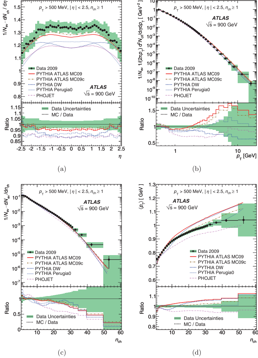
Fig. 2. – Inclusive-inelastic distributions of primary charged particles in the kinematic range p_T > 500 MeV and |\eta| < 2.5 in data at a centre-of-mass energy of \sqrt{s} = 900 GeV.
