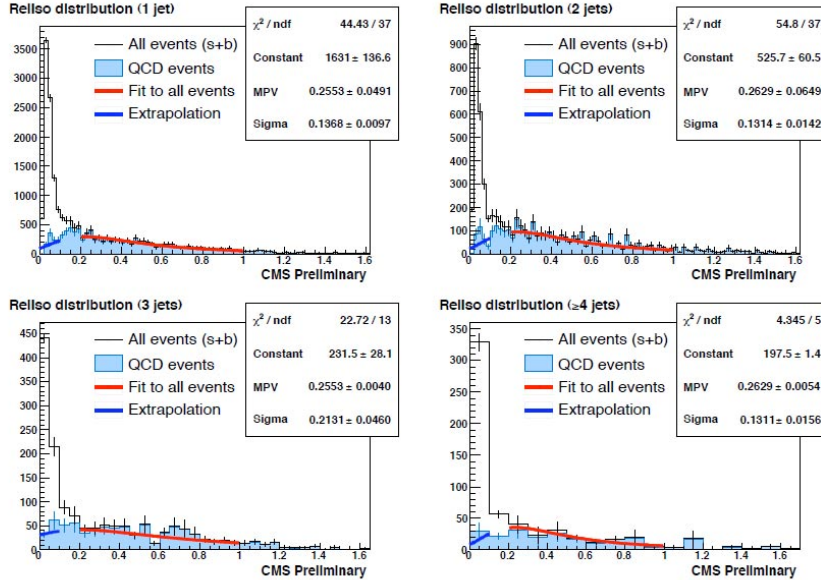
Fig. 2. – The reIso distributions for all events (unfilled histogram), and QCD events only (filled histogram). The fit using a Landau function in the range 0.2 < \text{reIso} < 1.0 is shown, together with the extrapolation into the signal region ( reIso < 0.1). The fit is carried out separately for samples with different jet multiplicities, and the MPV values from the 1 and 2 jet multiplicity fits are used to constrain this parameter for higher multiplicity fits [2].
