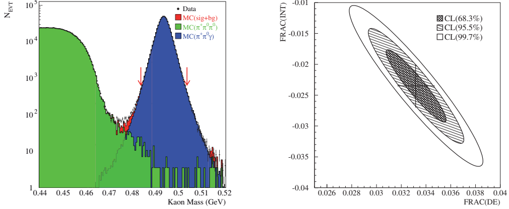
Fig. 1. – Left: kaon mass distribution for K^\pm \rightarrow \pi^\pm \pi^0 \gamma candidates. Right: contour plot in the DE INT plane.
