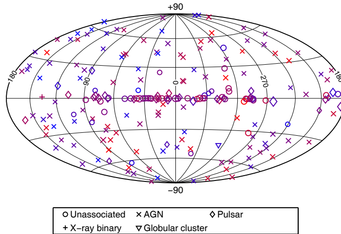
Fig. 3. – Location of the LAT Bright Sources [17].
