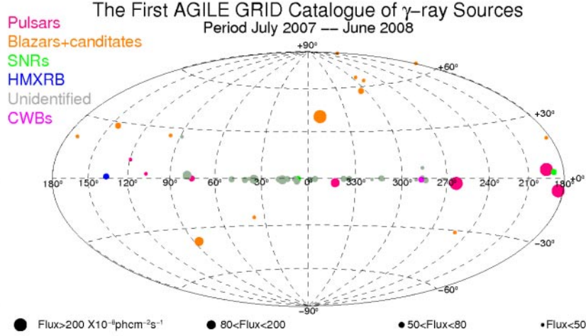
Fig. 2. – The First AGILE-GRID Catalog of high-confidence sources [11].
