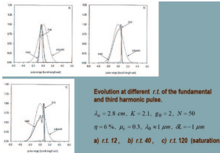
Fig. 5. – Intra-cavity evolution of a FEL oscillator operating at 1 μm.
