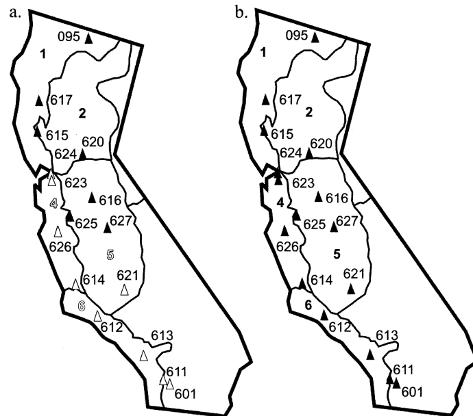
Fig. 1. – Maps showing climate divisions (1, 2, 4, 5, and 6) and locations of tree-ring chronology sites with site numbers (triangles). a) For La Niña years, sites with above average growth are indicated with dark triangles and with below average growth by light triangles. Divisions with above average winter precipitation are indicate with bold type and with below average winter precipitation with light type. b) For El Niño years, sites with above average growth are indicated with dark triangles and with below average growth by light triangles. Divisions with above average winter precipitation are indicate with bold type and with below average winter precipitation with light type.
