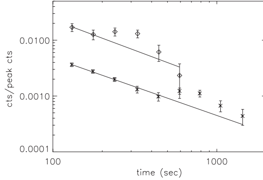
Fig. 1. – Average ratio of the flux with respect to the peak flux as a function of time since the GRB peak for the sample of 400 GRB studied by ref. [15]. Bright (asterisks) and dim (diamonds) GRB are represented. The solid lines show the best power-law fits to the decay. The excesses with respect to these fits in both luminosity classes are significant at > 3\sigma .
