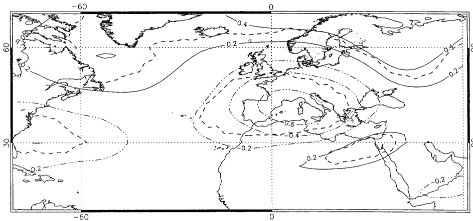
Fig. 8. – Pierson correlation coefficient between the precipitation SAI index and the 500 hPa geopotential height for the cold semester, averaged over the period 1948-1990. The thick dashed lines enclose areas at the 5% level, assessed by a Monte Carlo test.
