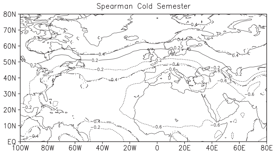
Fig. 10. – Correlation between Calabrian DSAI, in the cold semester, and the sea surface pressure, averaged over the period 1948-1990. The thick dot-dot-dashed lines enclose areas at a rejection level of 1%, assessed by a Monte Carlo test. Contours as in fig. 5a.
