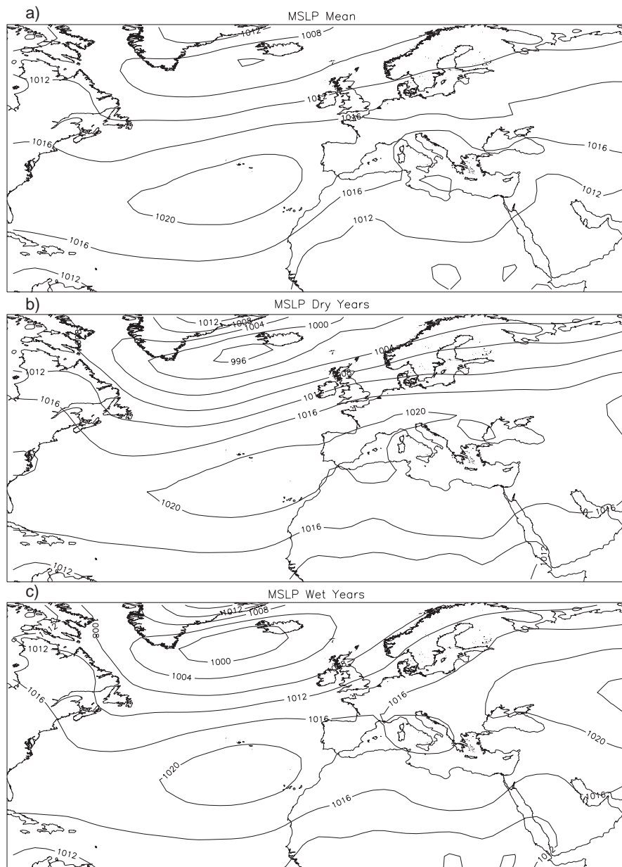
Fig. 7. – a) Mean sea level pressure averaged, for cold semesters, over 1948-1990. b) As in a) but for cold semesters below the 10th percentile (driest cold semesters). c) As in a) but for cold semesters above the 90th percentile (wettest cold semesters).
