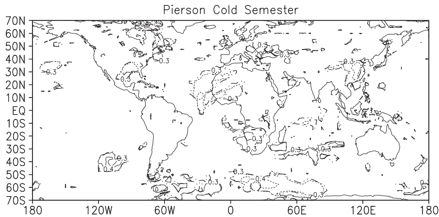
Fig. 11. – Correlation between precipitation over Calabria, during the cold semester, and SST, averaged over the period 1948-1990. The thick dashed lines enclose areas at the 10% level. The contour is 0.3.
