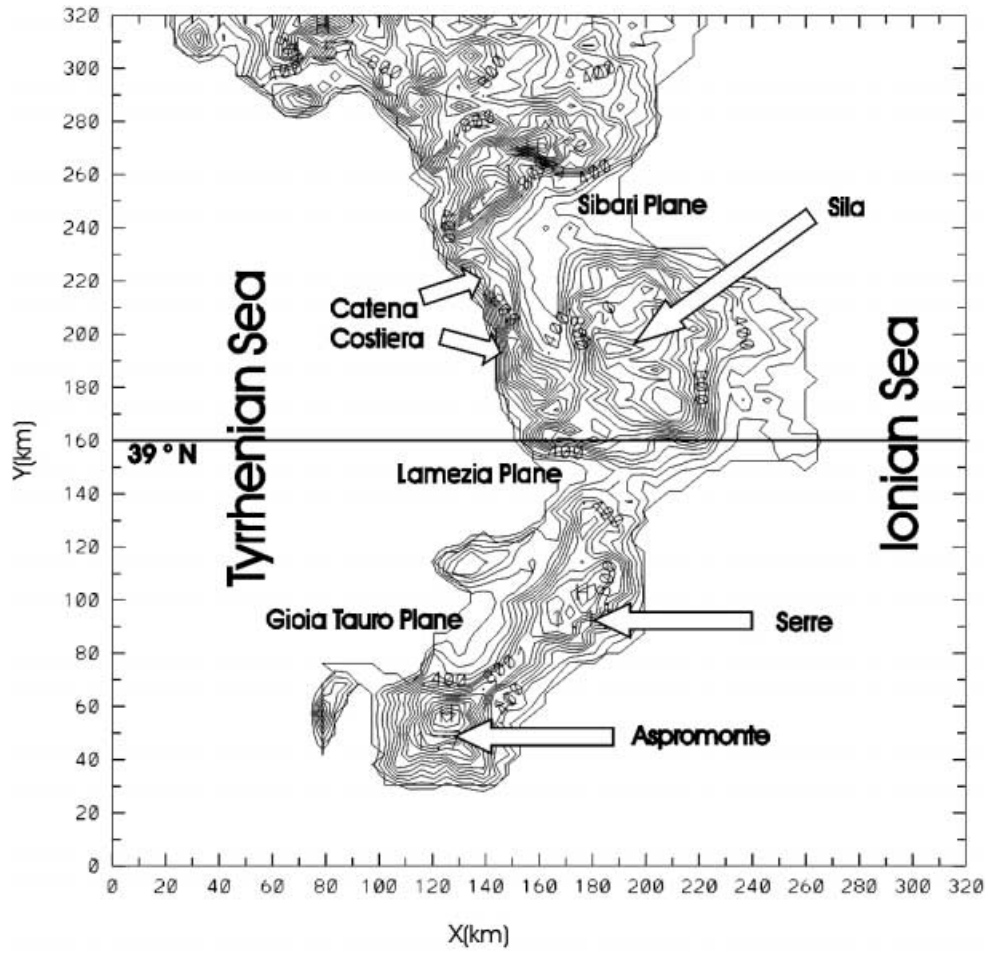
Fig. 1. – Calabria orography averaged over 10 km 2 . Main orographic features are also reported.
