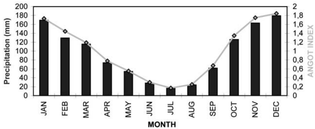
Fig. 2. – Monthly precipitation (left axis) and Angot index (right axis) averaged over 1921-1990.
