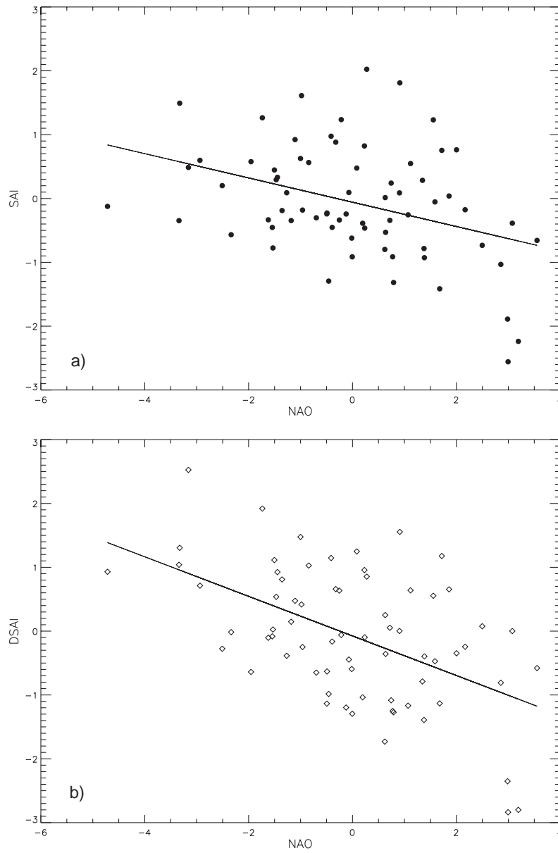
Fig. 4. – a) Linear regression of the NAO and SAI indices for the period 1921-1990. b) As in a) but for DSAI.
