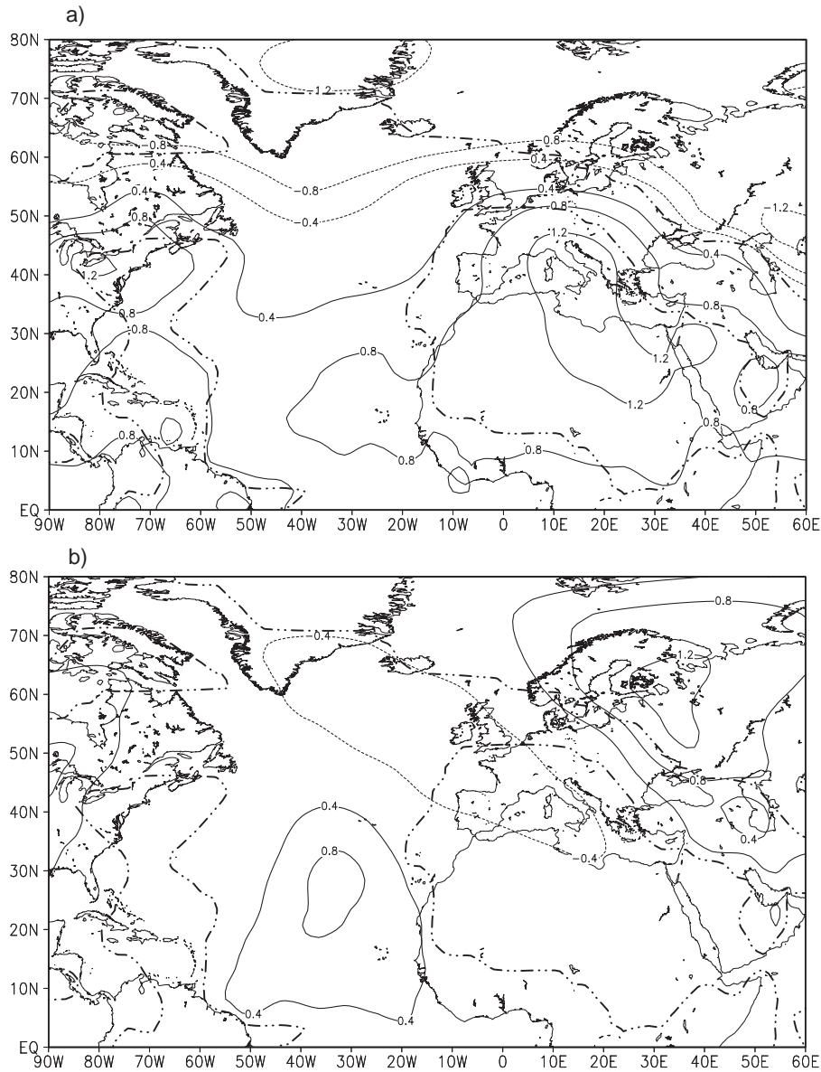
Fig. 6. – a) Sea level pressure anomaly averaged for the years with precipitation in the cold semester below the 10th percentile. Thick dot-dot-dashed lines enclose areas at the 5% level, assessed by a t -Student test. Absolute contour values from 0.4 to 1.2. The contour interval is 0.4. b) As in a) but averaged for the years above the 90th percentile.
