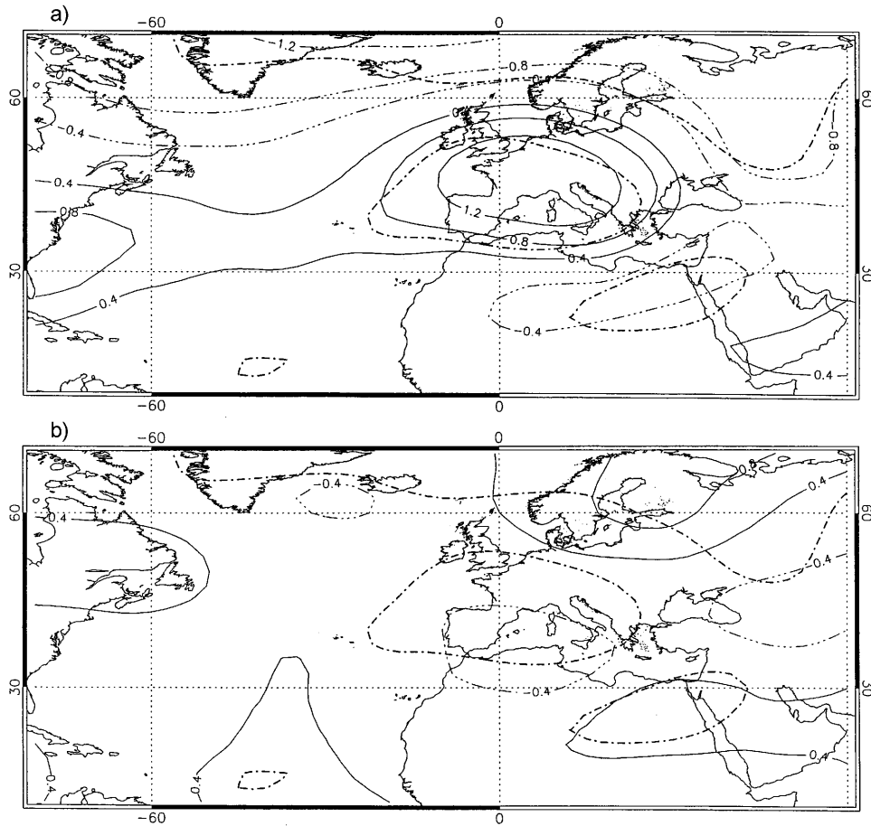
Fig. 9. – a) As in fig. 5a but for 500 hPa height. The thick dot-dashed lines enclose areas at the 10% level, assessed by a t -Student test. b) As in fig. 5b but for 500 hPa height.
