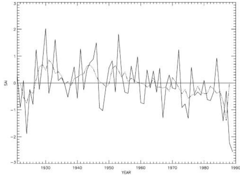
Fig. 3. – SAI index, averaged for all available stations, between 1921 and 1990. The five-years running mean is also reported.
