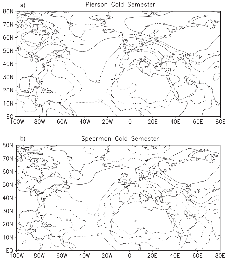
Fig. 5. – a) The Pearson correlation coefficients between SAI and sea level pressure for the cold semester, averaged over 1948–1990. The thick dot-dot-dashed lines enclose areas at the 5% level, assessed by a Monte Carlo test. Absolute contours values from 0.2 to 0.6. The contour interval is 0.2. b) As in a) but for the Spearman correlation coefficient.
