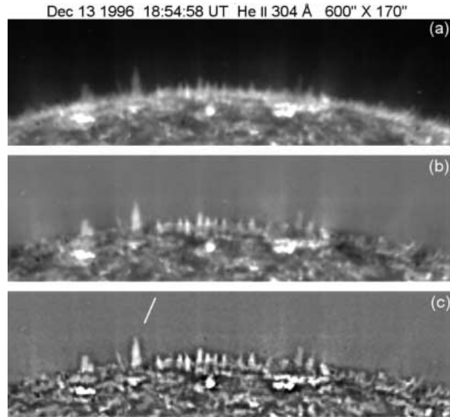
Fig. 3. – He II 304 Å images obtained on December 13, 1996 from EIT on board SOHO (ESA-NASA); (a) original image, (b) the same image corrected for limb darkening, (c) further enhanced using the Madmax operator.
