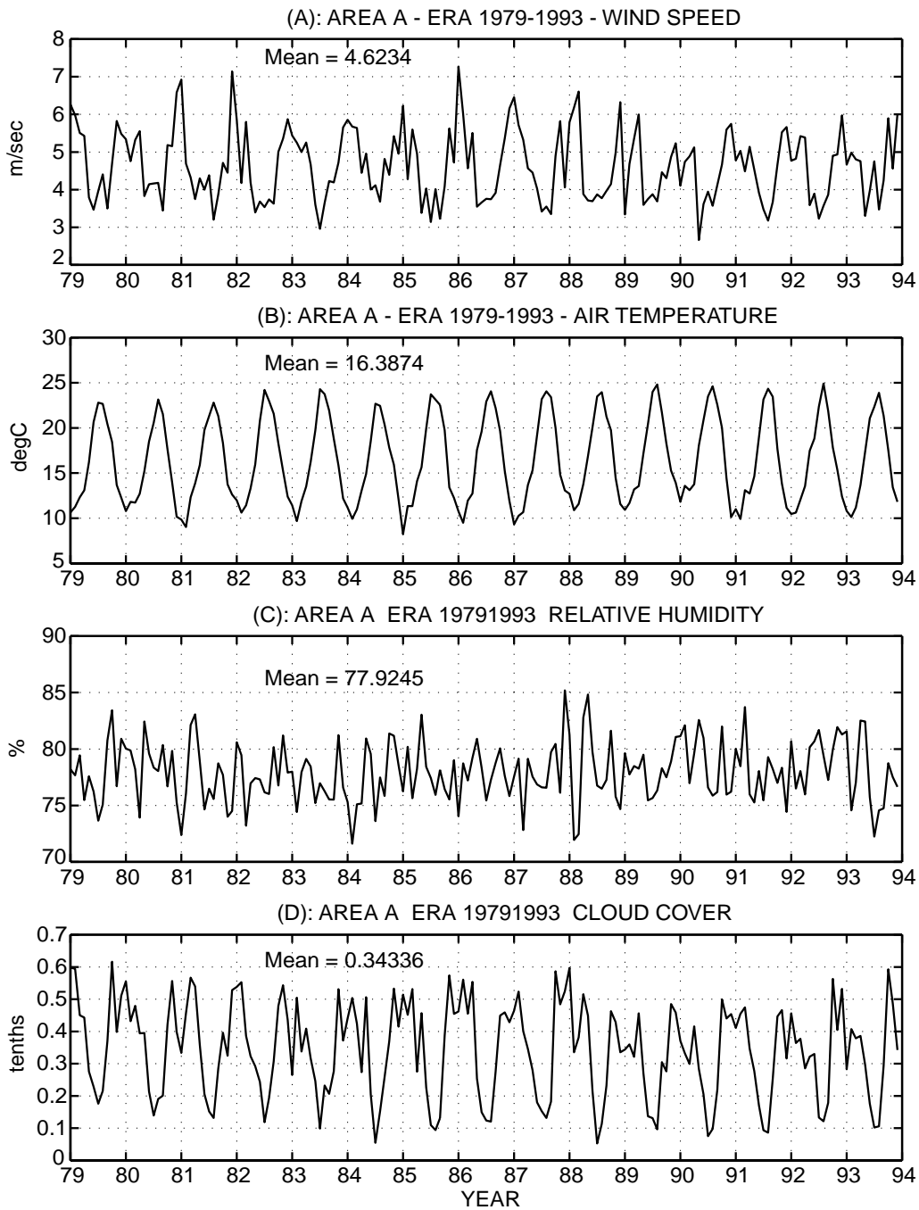
Fig. 4. – Surface means over the area A of ERA 1979-1993: wind speed /m/s (A); air temperature (°C) (B); relative humidity (%) (C); cloud cover (tenths) (D).
