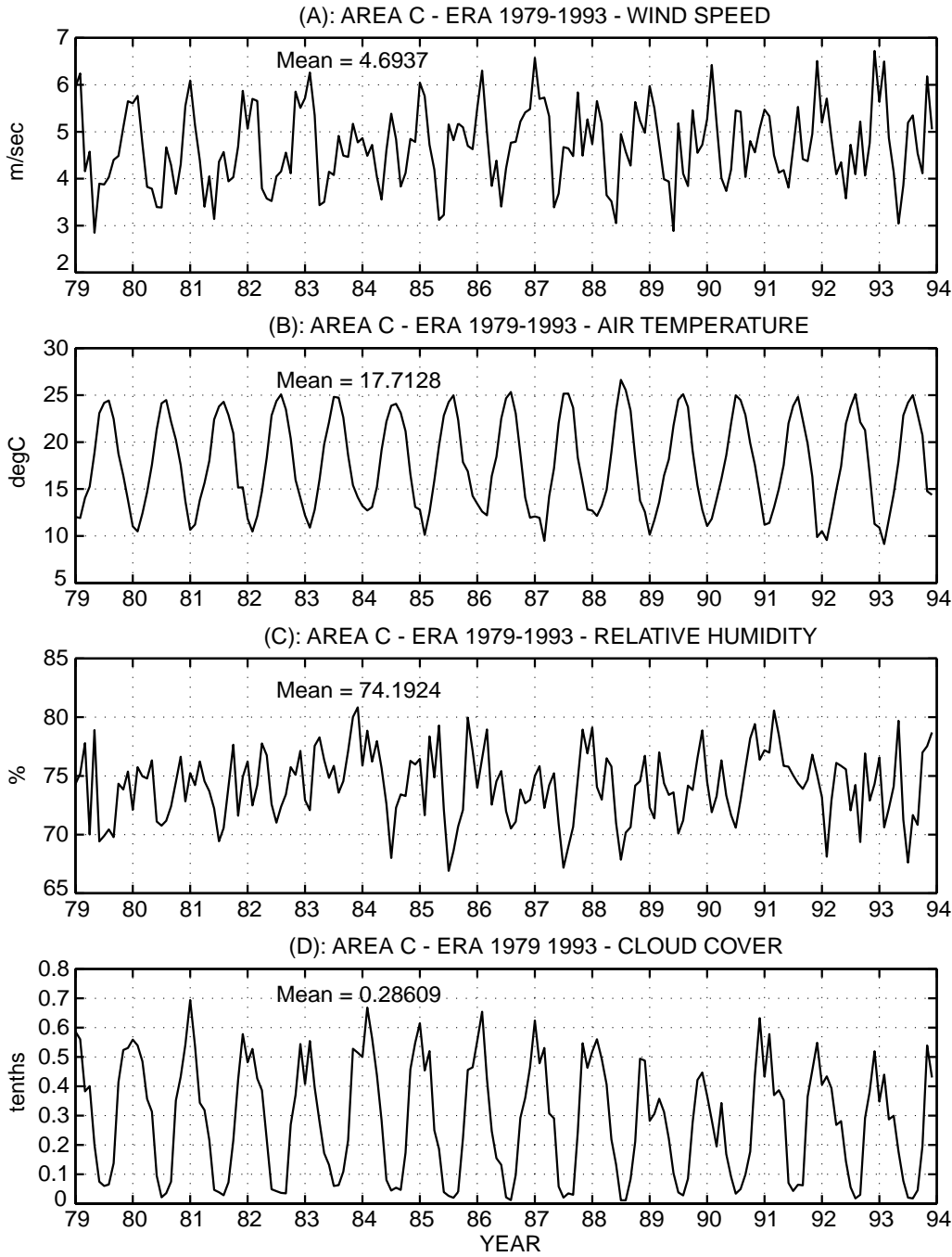
Fig. 6. – Surface means over the area C of ERA 1979-1993: wind speed (m/s) (A); air temperature (°C) (B); relative humidity (%) (C); cloud cover (tenths) (D).
