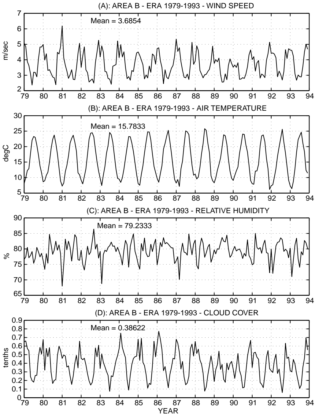
Fig. 5. – Surface means over the area B of ERA 1979-1993: wind speed (m/s) (A); air temperature (°C) (B); relative humidity (%) (C); cloud cover (tenths) (D).
