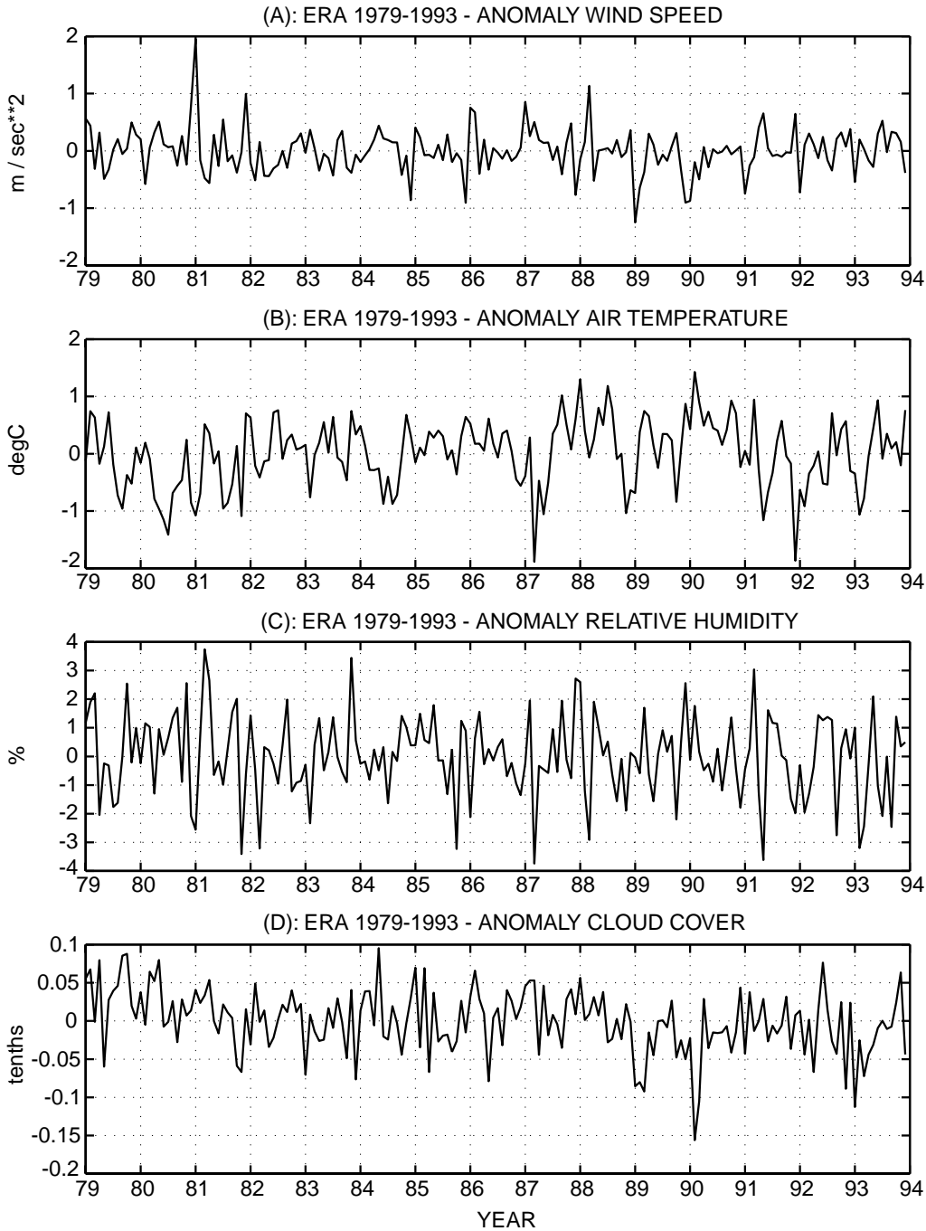
Fig. 2. – Med surface means of anomaly monthly ERA 1979-1993: anomaly wind speed (m/s) (A); anomaly air temperature (°C) (B); anomaly relative humidity (%) (C); anomaly cloud cover (tenths) (D).
