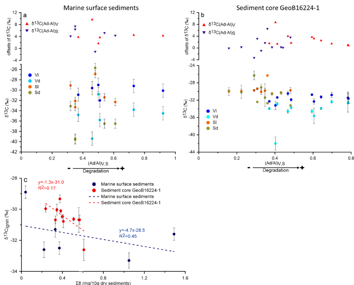
Figure 5.5. (a) \delta^{13}\text{C} values of aldehyde and acid phenols of V and S phenols (circles) and the offsets of \delta^{13}\text{C} values of aldehyde and acid phenols of V and S phenols, vs. corresponding Ad/Al ratios of V and S phenols (triangles) of marine surface sediments. (b) \delta^{13}\text{C} values of aldehyde and acid phenols of V ( \delta^{13}\text{C}(\text{Ad-Al})_{\text{V}} ) and S phenols ( \delta^{13}\text{C}(\text{Ad-Al})_{\text{S}} ), \delta^{13}\text{C}(\text{Ad-Al})_{\text{V}} vs. corresponding Ad/Al ratios of V and S phenols (circles) and the offsets of \delta^{13}\text{C} values of aldehyde and acid
