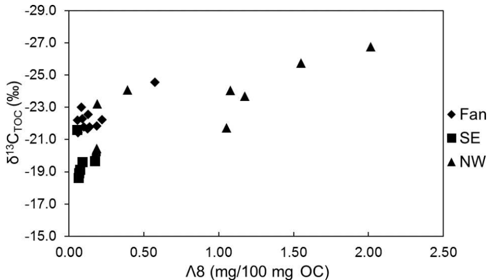
Figure 2.6. Stable carbon isotopic composition of total organic carbon ( \delta^{13}\text{C}_{\text{TOC}} ) vs. carbon-normalized lignin content ( \Lambda 8 ) for marine surface sediment samples from the Amazon continental margin.
