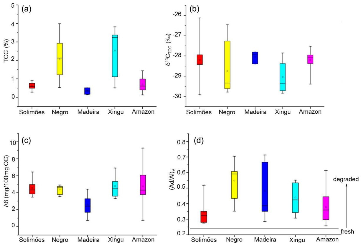
Figure 2.2. A) Total organic carbon (TOC) content, B) stable carbon isotopic composition of total organic carbon ( \delta^{13}C_{TOC} ), C) carbon-normalized lignin content ( \Lambda 8 ) and D) degradation index of lignin (Ad/Al)_v in different tributaries and in the Amazon mainstream. In D, (Ad/Al)_v \leq 0.24 suggests fresh vascular plant tissues, whereas (Ad/Al)_v > 0.24 reveals degraded plant material. See Table 2.1 and Fig. 2.1 for the location of the samples.
