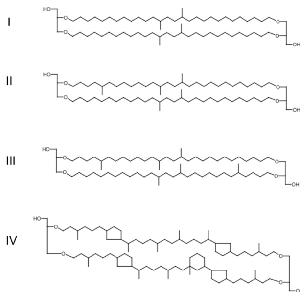
Figure 1.4. Structural formulas of branched GDGTs (I-III) and crenarchaeol (IV) (Zell et al., 2014).
