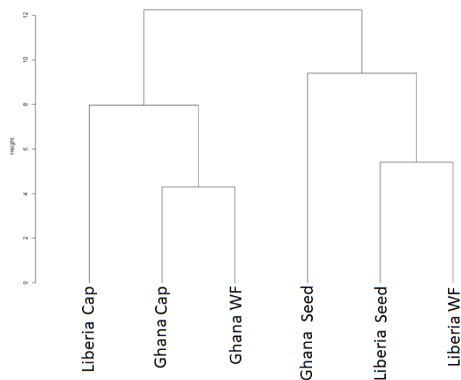
Figure 1. Cluster analysis of the essential oil chemical composition of Xylopi a aethi opica whole fruits (WF), and their parts (Cap, capsules) from Ghana and Liberia.
