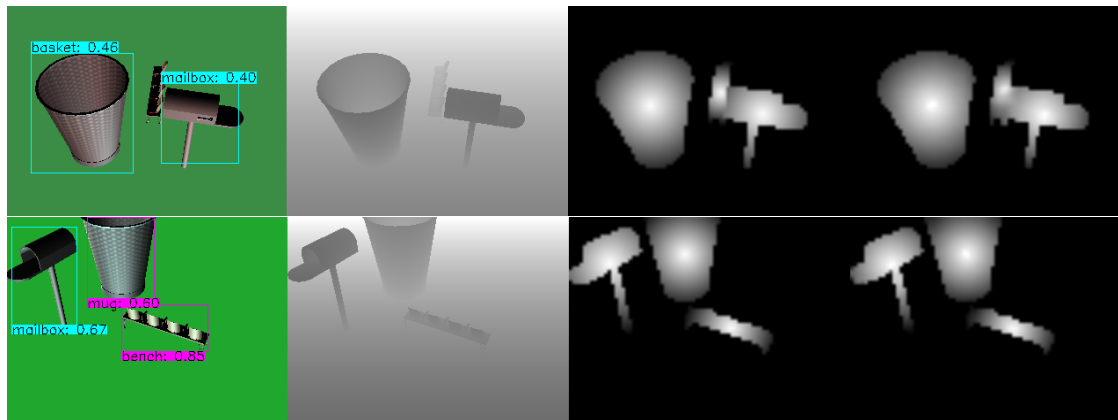
Figure 11. Prediction made with our extended YOLOv3 network. Left to right: (1) Input color image with predicted object instances; (2) Input depth frame; (3) Upscaled to 320x240 ground truth mask; (4) Predicted mask upscaled to 320x240. Same object is being treated as two distinct classes due to lack of cues for the artificial neural network of what the specific object may be due to scenes being generated randomly.
