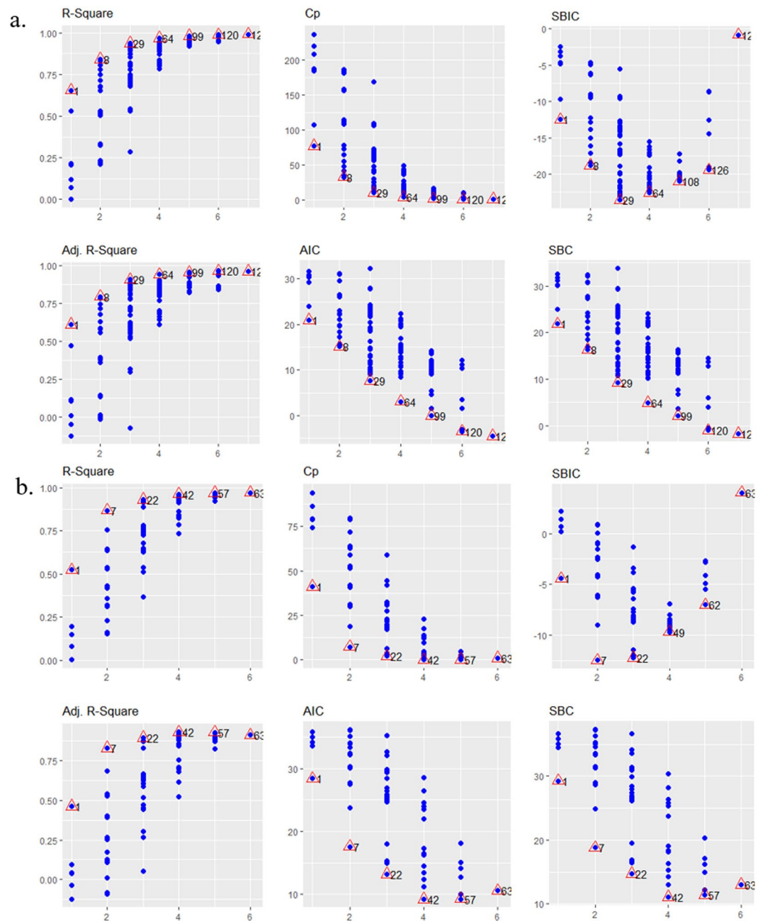
Figure 5. Pedo-transfer functions. (a), All possible PTFs for predicting \text{Log}(K_v) . The triangles indicate the best subset PTFs and the overall model numbers. (b), All possible PTFs for predicting \text{Log}(K_v, DA) . The triangles indicate the best subset PTFs and the overall model numbers.
