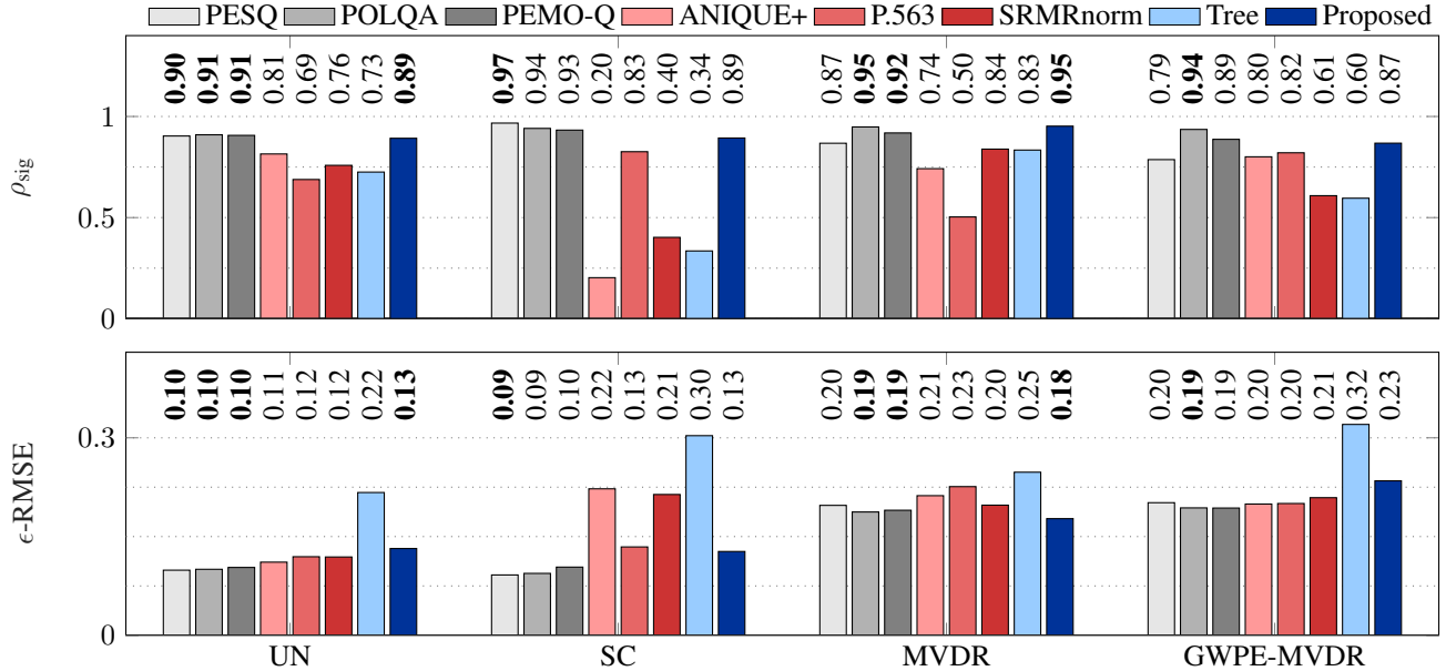
Fig. 5. Performance of the considered measures in terms of \rho_{\text{sig}} (top) and \epsilon - \text{RMSE} (bottom). The labels along the x-axis denote the category of algorithms included in training and testing sets. Numbers in bold typeface denote the best attained performance (statistically indifferent) per considered category of algorithm.
