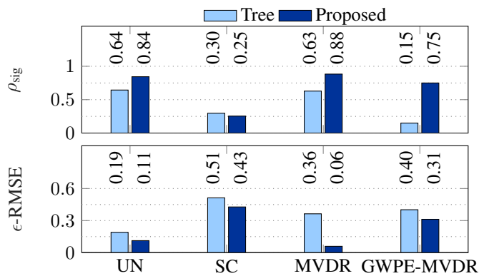
Fig. 8. Performance of the considered measures in terms of \rho_{\text{sig}} (top) and \epsilon - \text{RMSE} (bottom). The labels along the x-axis denote the category of algorithms included in testing sets while other categories were included in training.
