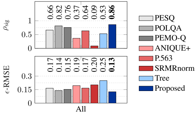
Fig. 6. Performance of the considered measures in terms of \rho_{\text{sig}} (top) and \epsilon -RMSE (bottom). All considered categories of algorithms were included in both training and testing sets. Numbers in bold typeface denote the best attained performance (statistically indifferent).
