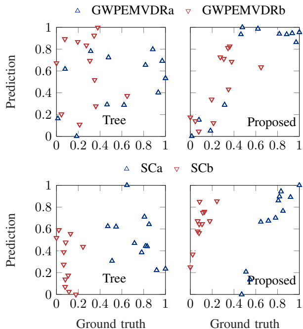
Fig. 9. Scatter plot of the predicted speech quality over ground truth data for Tree (left) and the proposed measure (right) when using a testing set of signals processed using either GWPE-MVDR (top) or SC (bottom). Scores are normalized to range between 0 and 1.
