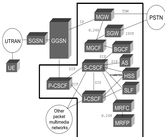
Fig. 1. IMS architecture overview
