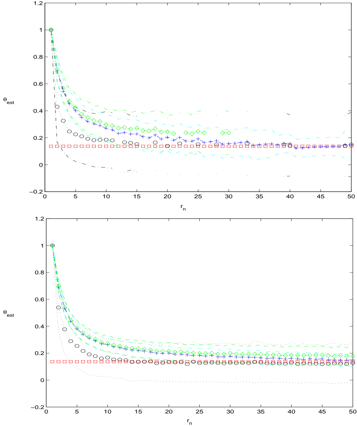
Figure 6.2. Estimated values of the extremal index for the doubly stochastic model with \psi = 0.9 and \eta = 0.7 . The extremal index is \theta = 0.137 plotted by \square line. The partitions r_n considered are in the range [1, 50] . \tilde{\theta}_n is represented by (\dots) and o ; the corresponding standard deviation is plotted with (\dots) . The logs method \hat{\theta}_n^{(1)} is represented with (- - -) and \diamond . The standard deviation with (\dots) . The blocks method \hat{\theta}_n^{(2)} with (\cdot - \cdot -) and + , and (\cdot - \cdot -) for the standard deviation. The sample sizes are n = 200 and n = 1000 respectively. m = 100 simulations are used. The threshold sequence is \hat{u}_n = x_{(n-k)} with k = \sqrt{2n} .
