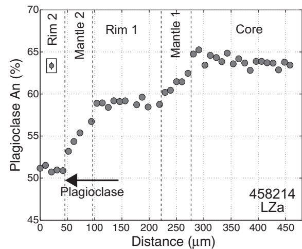
Fig. 10. Examples of Type I plagioclase grains in LZa showing a core surrounded by two different mantles of decreasing An content and two rims buffered to a constant composition (rim 1: \text{An}_{55-58} ; rim 2: \text{An}_{50-51} ).
