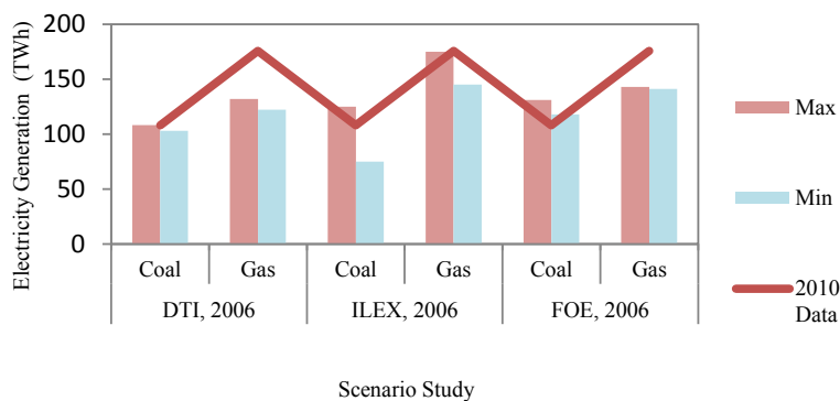
Fig.3: Projected Coal & Gas Generation Comparison for 2010
