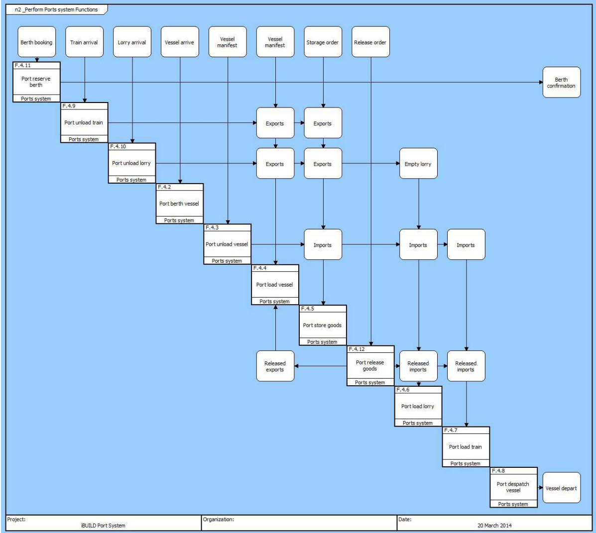
Figure 3: N² Diagram for a Hypothetical Port with Principal Functions and Related Interdependencies
