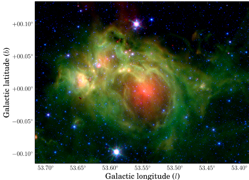
Figure 19. Star-forming region Sh 2-82 as seen in the mid-infrared by the Spitzer Space Telescope . The mosaic is composed of the 24 \mu\text{m} (red), 8.0 \mu\text{m} (green), and 4.5 \mu\text{m} (blue) bands. The image reveals a bubble-shaped structure which surrounds the HII region that is seen in the IPHAS mosaic which spans the same region (Fig. 18). This structure has previously been labelled as N115 in the catalogue of Churchwell et al. (2006), and could be a possible site of triggered star formation (Kendrew et al. 2012; Thompson et al. 2012).
