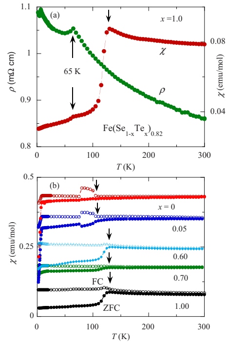
FIG. 4. (Color online) (a) Magnetic susceptibility \chi and resistivity \rho as a function of temperature for the sample with x = 1.0 . An anomaly near 65 K is observed in both measurements. The arrow near 125 K indicates the magnetic anomaly temperature, below which \chi exhibits marked irreversibility between FC and ZFC cooling histories as shown in panel (b). (b) Magnetic susceptibility \chi(T) measured following FC and ZFC cooling histories for the samples with x = 0, 0.05, 0.6, 0.7 , and 1.0 . The transitions at low temperatures correspond to the superconducting Meissner effect. The Meissner effect is observed in all samples except for x = 1.0 .
