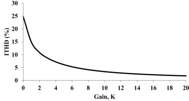
Fig. (8). ITHD versus active-power filter gain: Objective 2, Case 4
