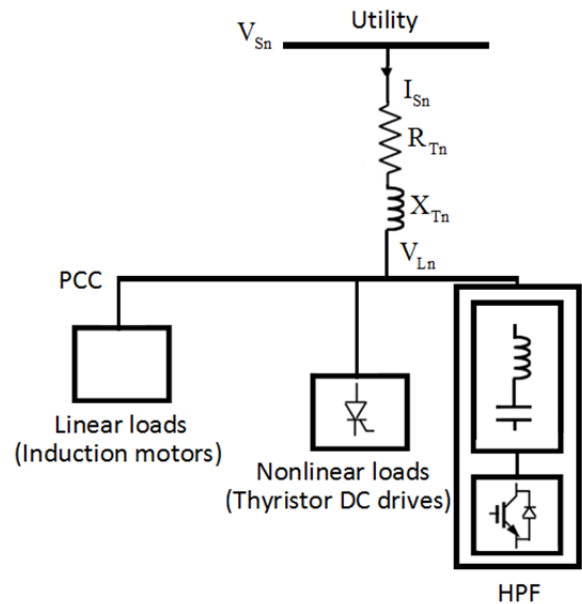
Fig. (1). Single-phase diagram of the proposed arrangement
