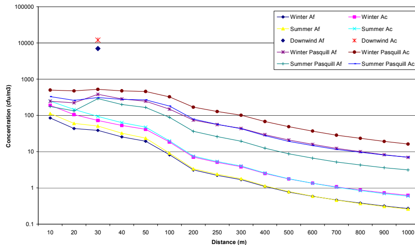
Figure 3. The influence of season and meteorological data on modelled predicted concentrations of A. fumigatus (Af) and actinomycetes (Ac).
