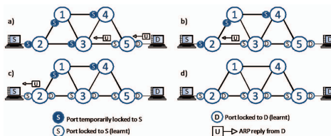
Figure 1. ARP-Path path confirmation with snooped ARP Reply
