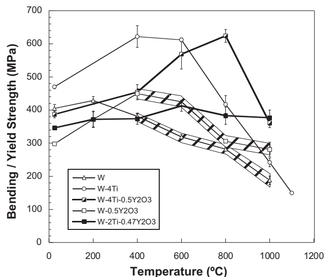
Fig. 1. Bending or yield strength of the samples tested in three-point bending. Shaded values stand for the yield strength at 0.2% of plastic strain (material with plastic deformation before fracture). Non shaded values stand for bending strength (tests with a linear response until fracture).
