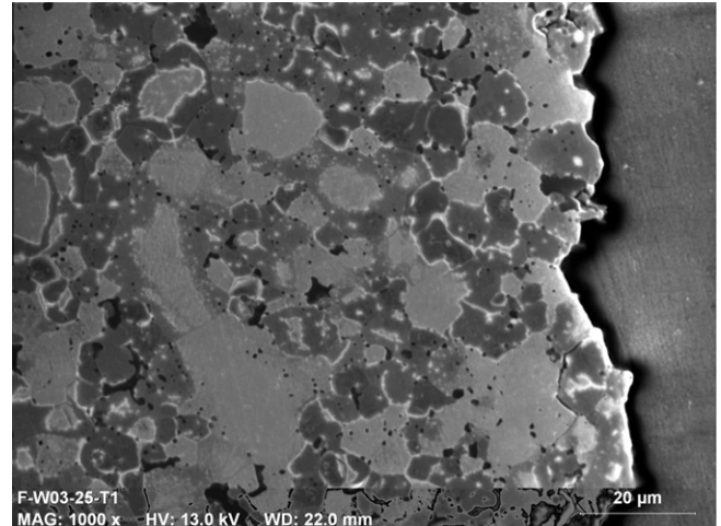
Fig. 4. Cross section showing the fracture surface profile in W-4% Ti-0.5% Y 2 O 3 alloy (bending tested at 25 °C). Sample etched with Murakami reagent.
