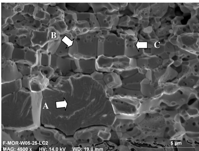
Fig. 3. SEM micrograph showing the fracture surface with intergranular porosity of W-2% Ti-0.47% Y 2 O 3 alloy (bending tested at 25 °C). Cleavage (A), aligned W grains (B) and porosity below the boundary grain (C).
