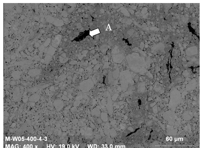
Fig. 5. Micrograph of W-2% Ti-0.47% Y 2 O 3 alloy bending tested at 400 °C (etched with Murakami reagent). (A) Ti pools.
