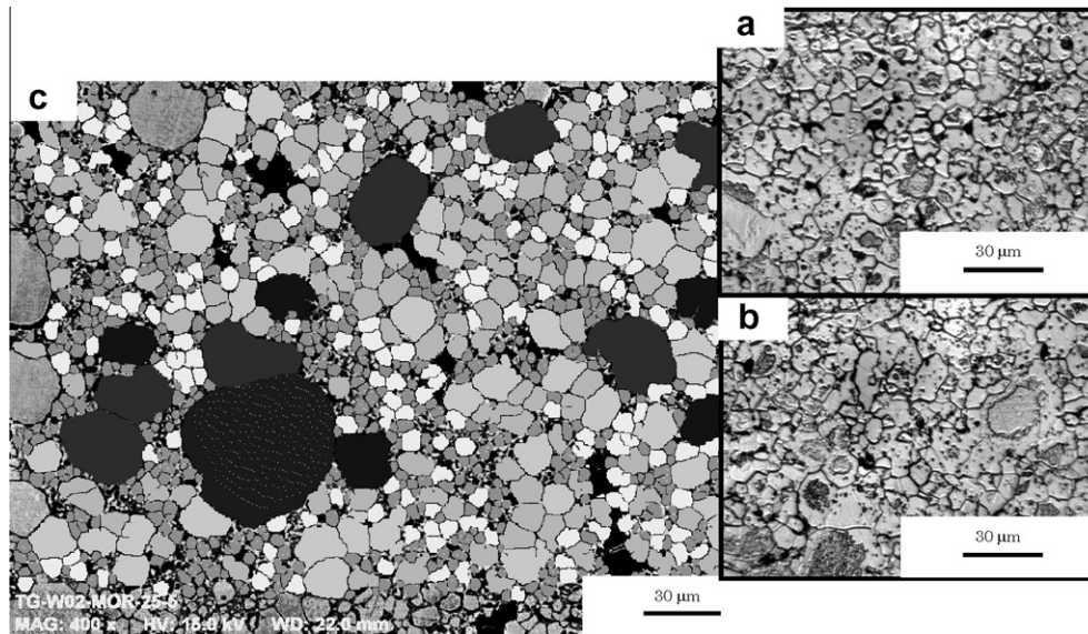
Fig. 6. Micrographs for grain size estimation. (a and b) W-4% Ti-0.5% Y 2 O 3 and (c) W-4% Ti (reference material).
