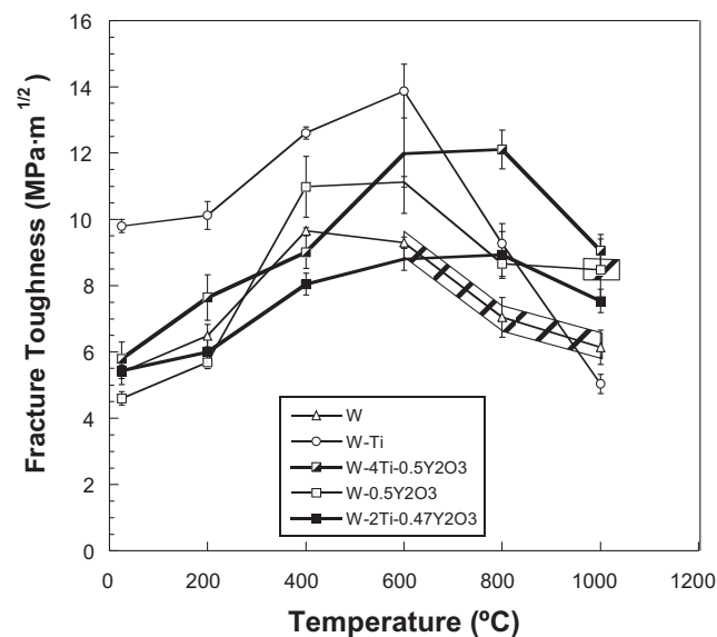
Fig. 2. Evolution of fracture toughness with test temperature. Shaded values stand for "apparent fracture toughness" (tests with substantial plastic deformation before maximum load).
