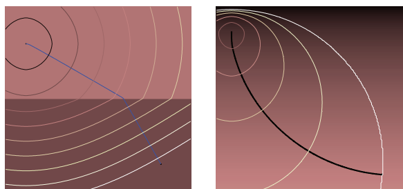
Figure 1. Hot road surface mirage: Light rays bending due to change of the refraction index in air with higher temperature (and lower refraction index) near the road surface.
