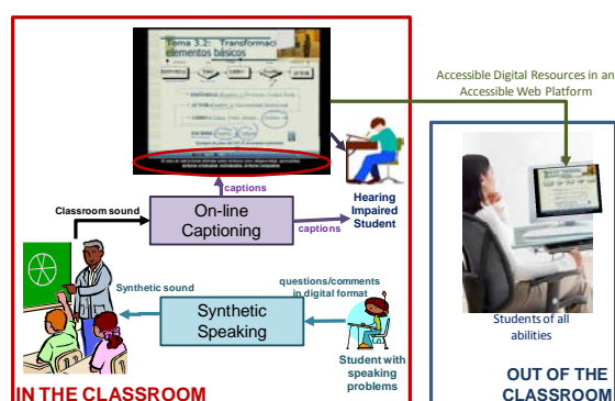
Figure 1. APEINTA architecture
