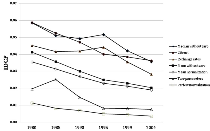
Fig. 3. A comparison of the IDCP term in absolute value after applying the different normalization procedures in the six yearly datasets.
