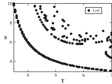
FIG. 3. Boundaries between areas of solutions with different periodicity. Proceeding away from the bottom left corner, dots indicate curves where the maximum Lyapunov exponent vanishes and separate regions where the asymptotic state is a fixed point, a period two orbit, a period four orbit, etc. The basic square lies outside the bottom left corner of the plot, in the fixed point region.
