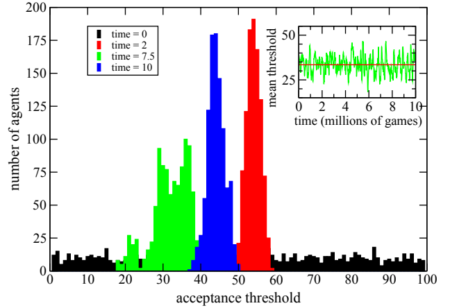
Fig. 1. Non-self-interested behavior establishes spontaneously in small populations. Population size is N = 1000 , the capital to be shared per game is M = 100 . Death and birth takes place after every game ( s = 1 ). Initial acceptance thresholds are distributed uniformly ( t_i = t_0 conditions lead to the same output). Plotted are the distributions of acceptance threshold at the beginning of the simulation and after 2, 7.5 and 10 million games. Inset: Mean acceptance threshold as a function of simulated time, is averaged over intervals of 10 000 games to reduce noise (in the raw data spikes appear that go above 50 or below 10). The red line in the inset is the average over all times of the mean, located at 33.45.
