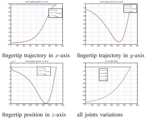
Fig. 3. Positions and angles obtained results using the MSDLS method with \Delta x_{max} = 1mm
