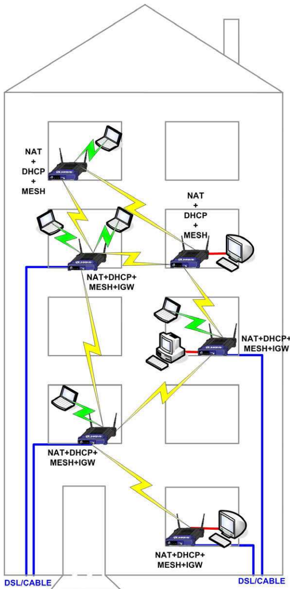
Fig. 1. Community wireless mesh scenario.
