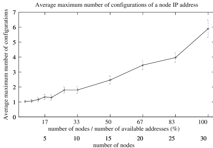
Fig. 7. Average maximum number of configurations of the IP address of a node (single-hop bootstrapping scenario).
