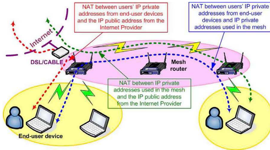
Fig. 2. Community WMN IP addressing approach.
