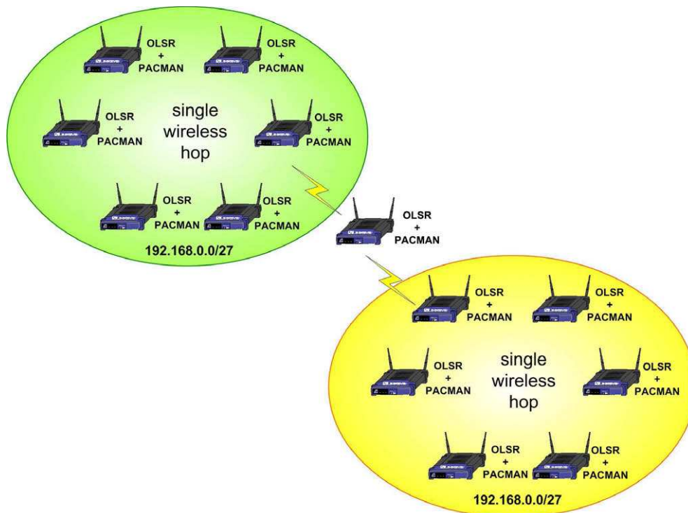
Fig. 11. Merging of two networks.
