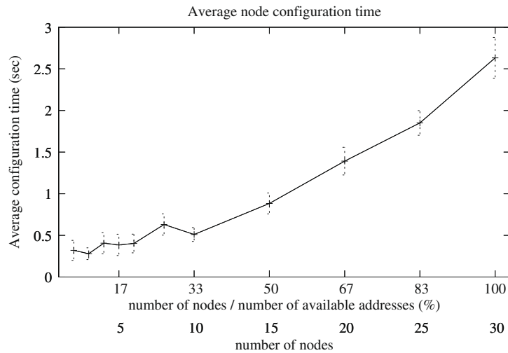
Fig. 5. Average node configuration time (single-hop bootstrapping scenario).
