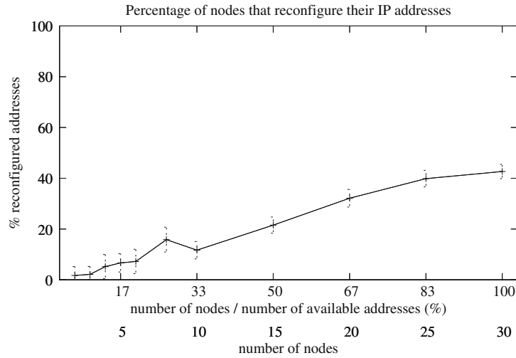
Fig. 8. Percentage of nodes that needed to reconfigure their IP address (single-hop bootstrapping scenario).
