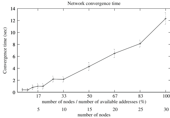
Fig. 4. Average network autoconfiguration convergence time (single-hop bootstrapping scenario).
