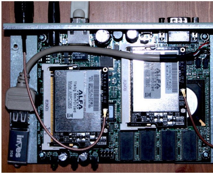
Figure 5.3: Hardware platform
