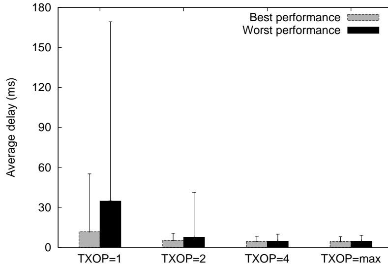
Figure 3.22: Delay performance for different TXOP.
