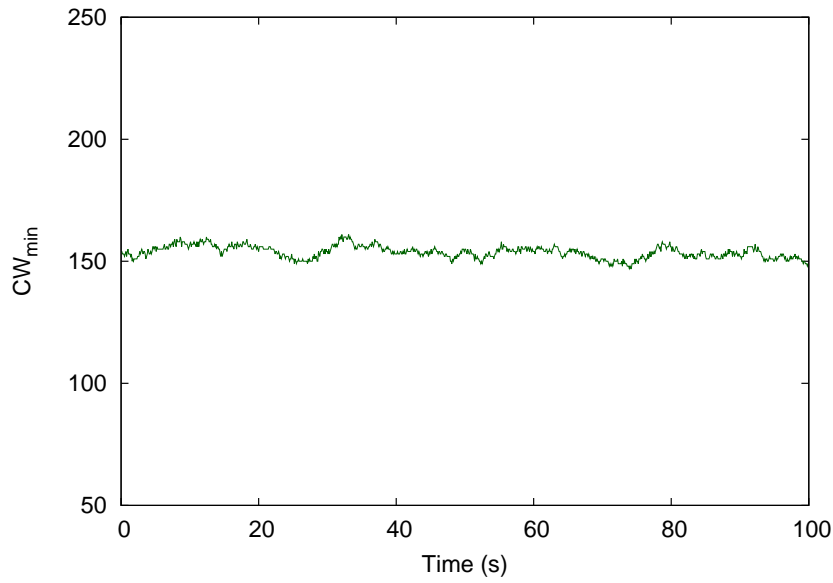
Figure 3.4: Stable configuration.
