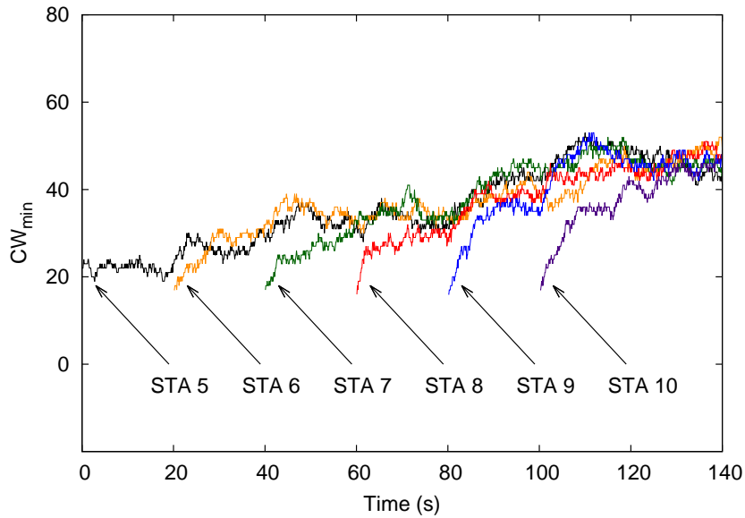
Figure 4.9: Convergence
