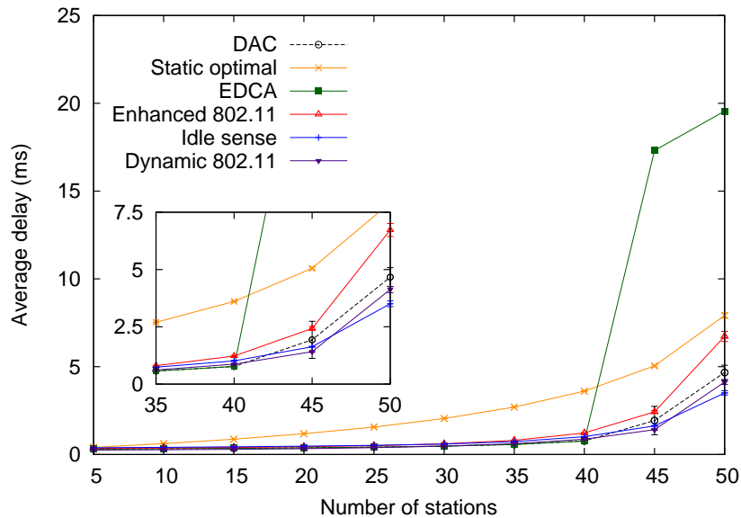
Figure 4.4: Non-saturation scenario
