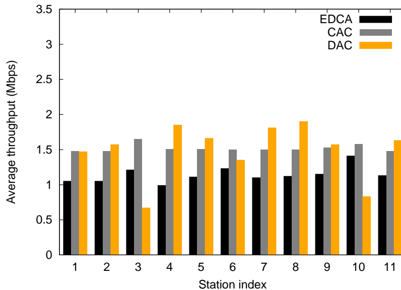
Figure 5.13: Throughput per station with quasi-homogeneous link qualities
