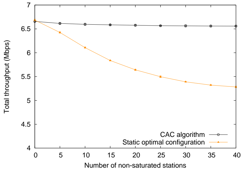
Figure 3.9: Bursty traffic.
