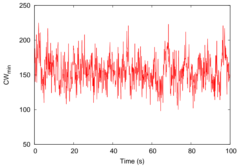
Figure 3.5: Unstable configuration.
