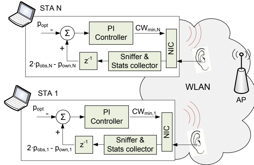
Figure 5.2: DAC algorithm
