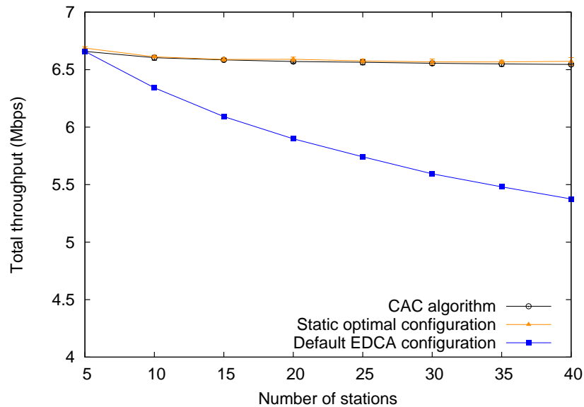
Figure 3.3: Throughput performance.
