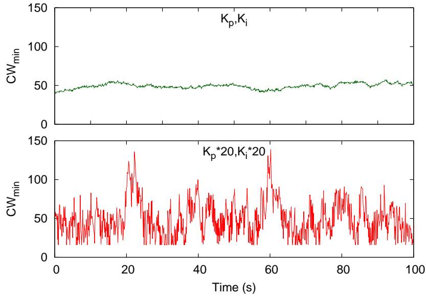
Figure 4.10: Stability validation
