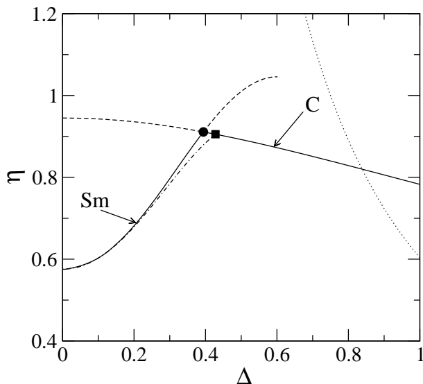
FIG. 1: N-Sm and N-C spinodals obtained with the second virial approximation of the direct correlation function. The solid line always show the first phase (labelled in the figure) which bifurcates from the uniform nematic phase N. Length-polydispersity is taken as a Schultz distribution function, although only the N-Sm bifurcation line depends on this choice. The dot-dashed line shows the N-Sm spinodal obtained with the choice (42) for the polydispersity distribution. The filled circle and square show, respectively, the crossover polydispersity values \Delta_{\times} arising from this two distribution functions. Finally, the dotted line shows the location of the N-N demixing spinodal.
