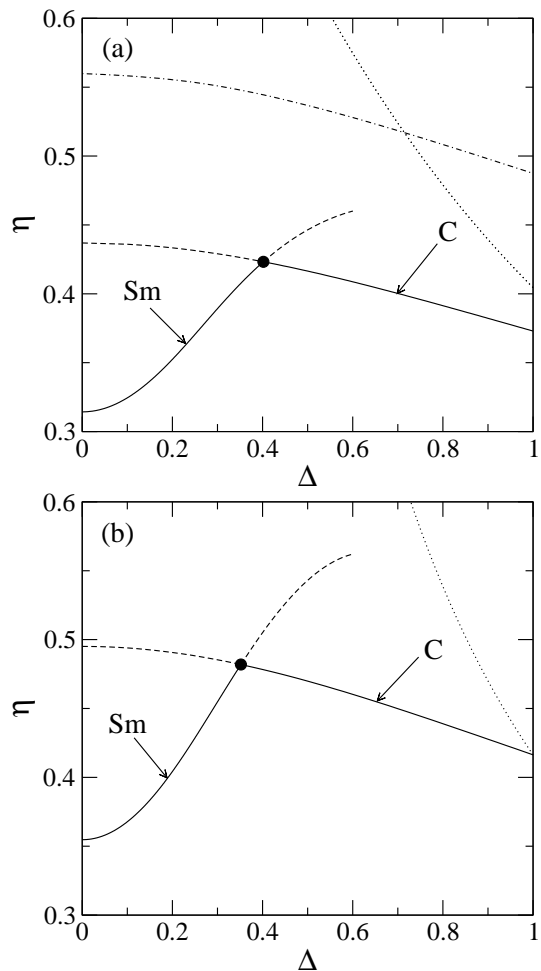
FIG. 2: N-Sm and N-C spinodals obtained with the fundamental-measure density functional proposed in ref. [45] (a) and with the third virial approximation (b). Lines and dot mean the same as in fig. 2. The dot-dashed line in (a) shows the N-C spinodal arising from the fundamental-measure density functional arising from Rosenfeld’s approximation for the hard disk fluid. Notice that it never meets the N-Sm bifurcation line.
