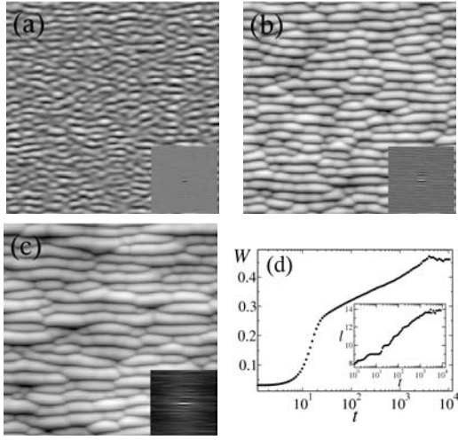
FIG. 3: Numerical integration of Eq. (7) for parameters as in Fig. 1, except for \lambda_x^{(1)} = 1 . Top views for t = 10, 106, 953 (a), (b), and (c), respectively. (d): Surface roughness W(t) for the same simulation. Inset: l(t) for the same system, showing marginal coarsening. All units are arbitrary.
