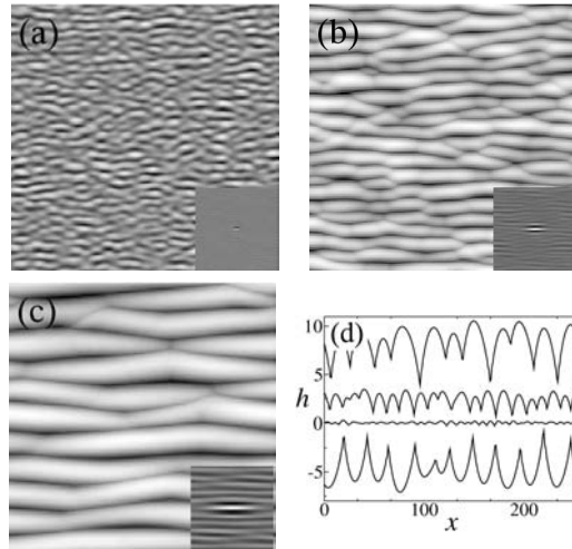
FIG. 1: Numerical integration of Eq. (7) using \nu_x = 1 , \nu_y = 0.1 , \Omega_x = 1 , \Omega_y = 0.5 , \xi_i = 0.1 , \lambda_x^{(1)} = 0.1 , \lambda_y^{(1)} = 5 , \lambda_{i,j}^{(2)} = -5 , \mathcal{K}_{i,j} = 1 . Top views for t = 10, 106, 953 (a), (b), and (c), respectively. Insets are height autocorrelations. All units are arbitrary. (d): Top to bottom, side cuts of (c), (b), (a), and grooves obtained for sign-changed \lambda_{x,y}^{(1)} and \lambda_{i,j}^{(2)} . Curves have an artificial offset.
