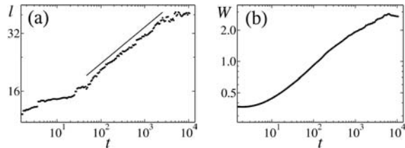
FIG. 2: Ripple wavelength \ell(t) and surface roughness W(t) for parameters as in Fig. 1. The straight line represents \ell \sim t^{0.19} . All units are arbitrary.
