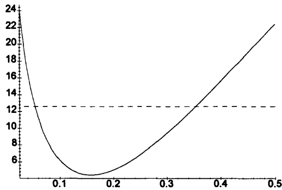
FIG. 2. Likelihood ratio for CPCE as a function of \epsilon .
