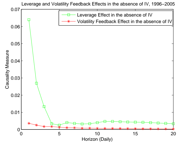
Figure 4. Leverage and volatility feedback effects, with implied volatility as auxiliary variable [trivariate models (r, RV, IV) and (r, RV, IV - RV) ] and without implied volatility [bivariate model (r, RV) ]. January 1996 to December 2005.
