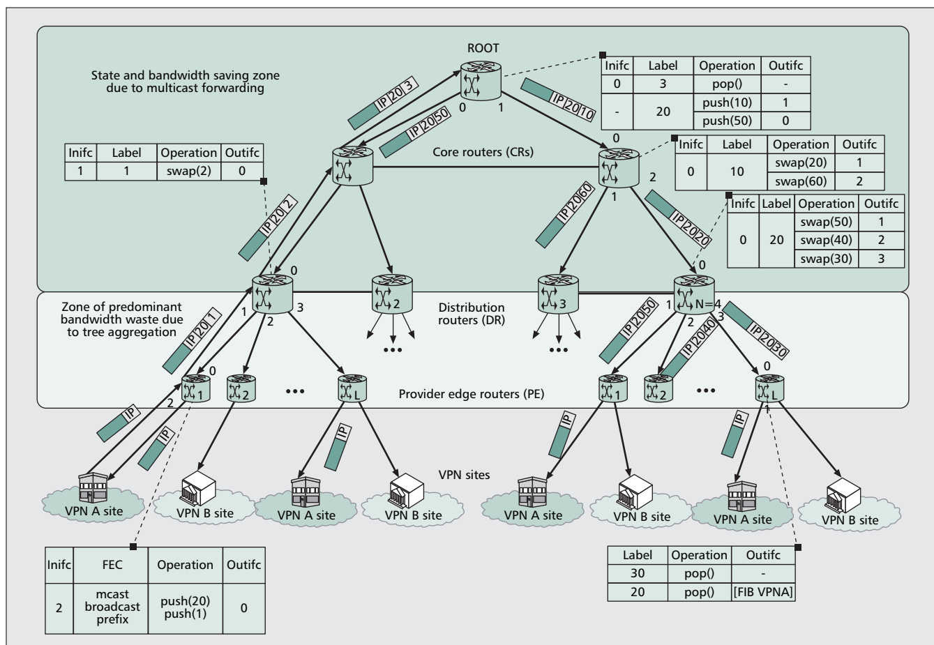
■ Figure 3. Network topology with aggregated multicast tree example.
