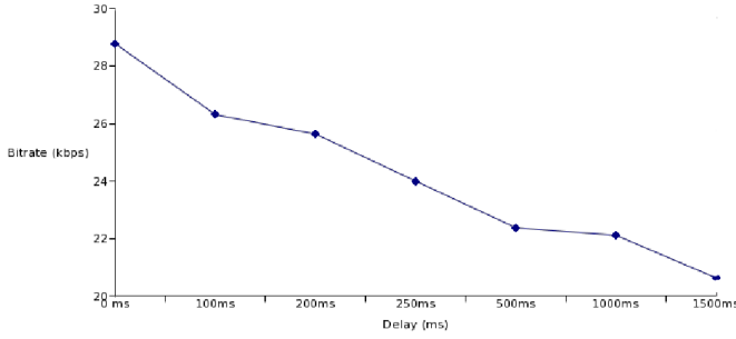
Fig. 3. MR's operation: Throughput vs Added Delay
