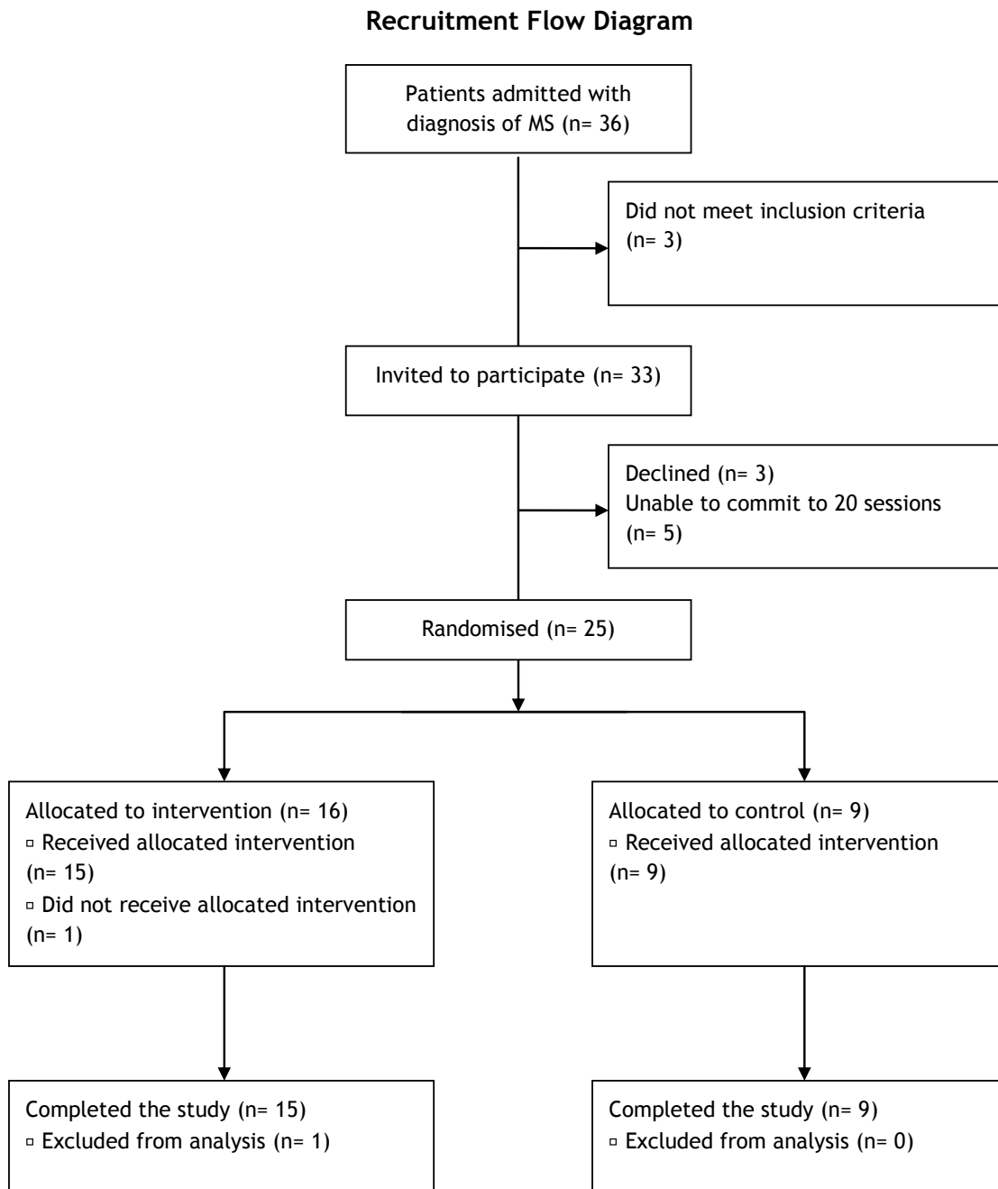
Figure 1 Consort diagram
