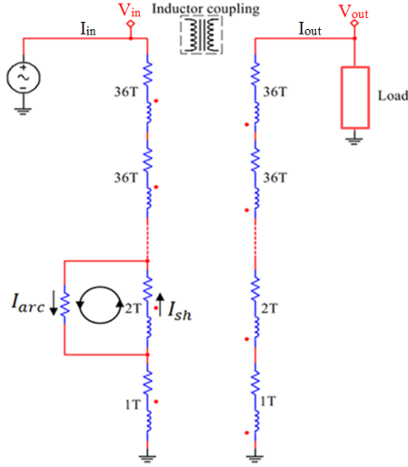
Fig. 2 PSPICE simulated transformer with two turns short-circuited
