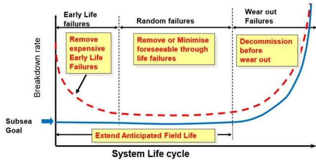
Figure 2. A perspective of the reliability bathtub curve for subsea application (Strutt &amp; Wells, 2014).
