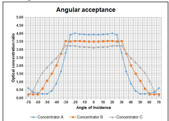
Figure 6. Angular acceptance of Concentrators A, B, C
