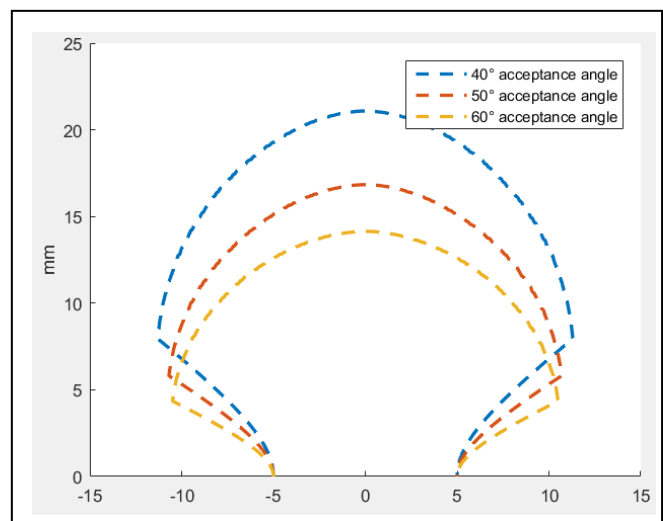
Figure 2. From highest to lowest: side view of Concentrators A, B, C
