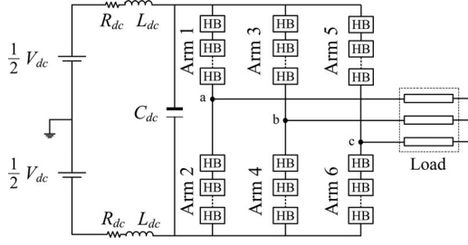
Fig. 3. Three-phase Q2LC.
