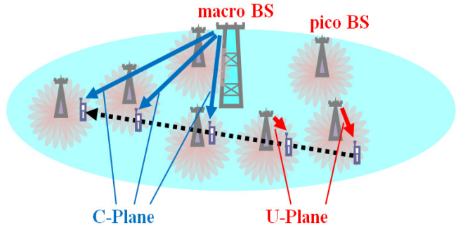
Fig.9. C-MoDe Operation.
