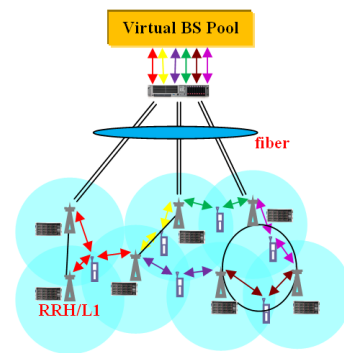
Fig. 4. Partially Centralized C-RAN.
